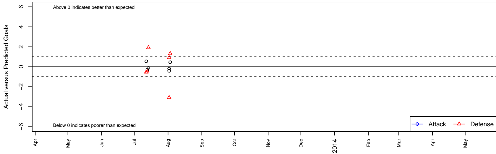
WA Rush Nero B95 Dots are actual minus expected GF (blue circles) and GA (red triangles). Blue line is smoothed change in attack strength. Red is smoothed change in defense strength.
